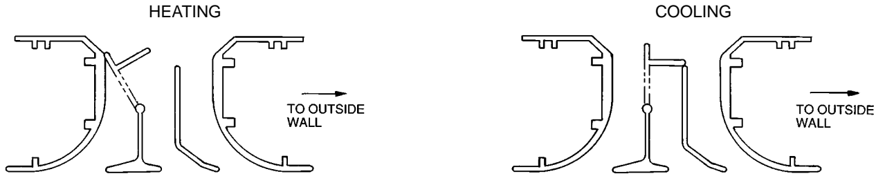
Fig. 7 — Director Diffuser
